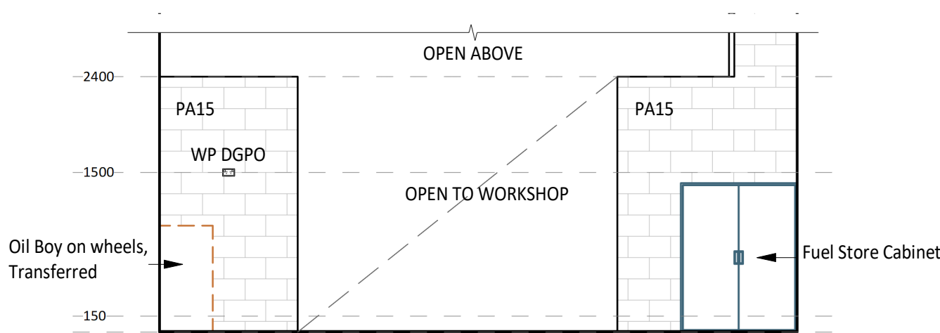
3 ELEVATION DETAIL 60-006 1 : 50
