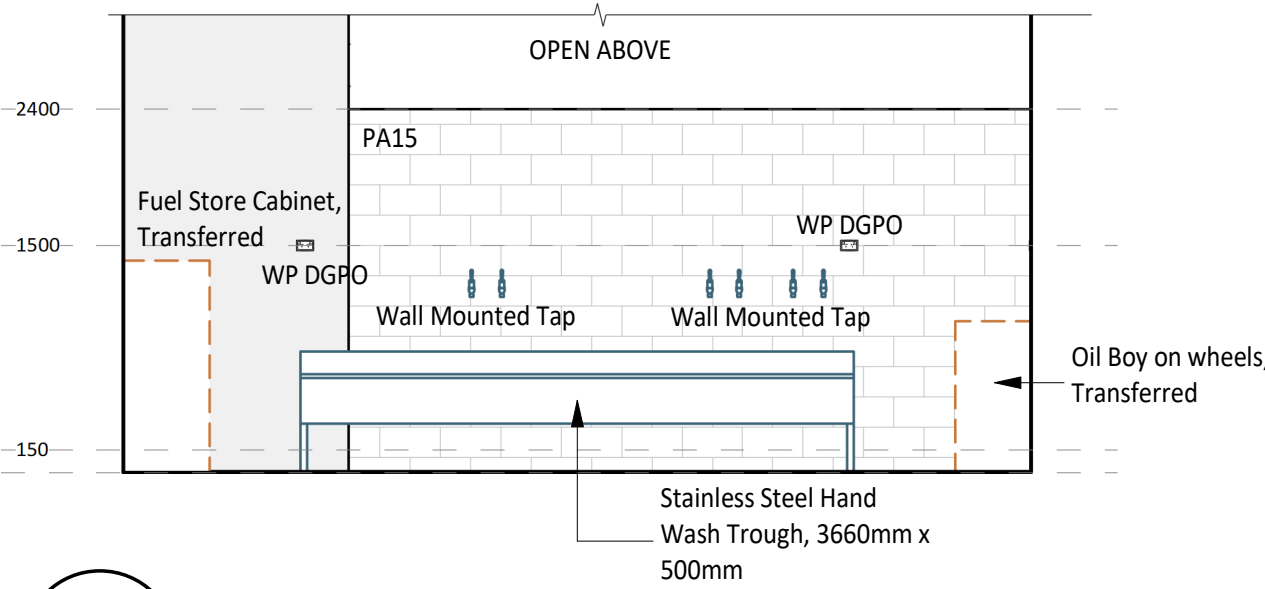
2 ELEVATION DETAIL 60-006 1 : 50
