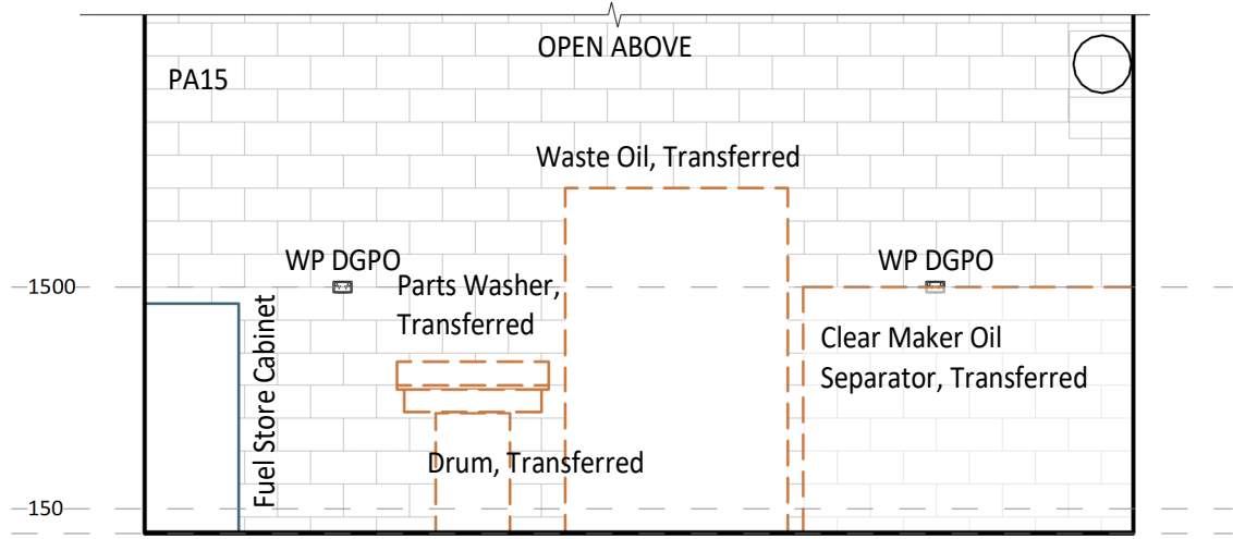
4 ELEVATION DETAIL 60-006 1 : 50
