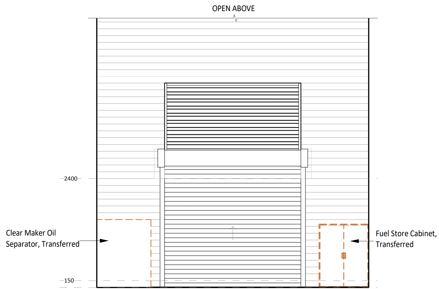
5 ELEVATION DETAIL 60-006 1 : 50
